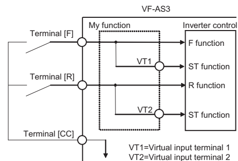
Fig. 5-2 Block diagram for Example 1
