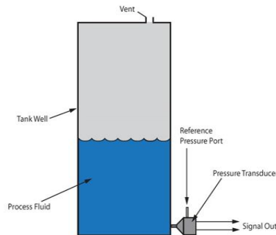
Figure 4: Differential pressure sensors monitor for the process fluid level by measuring the total pressure difference between the fluid at the bottom of the tank and the vessel pressure.
