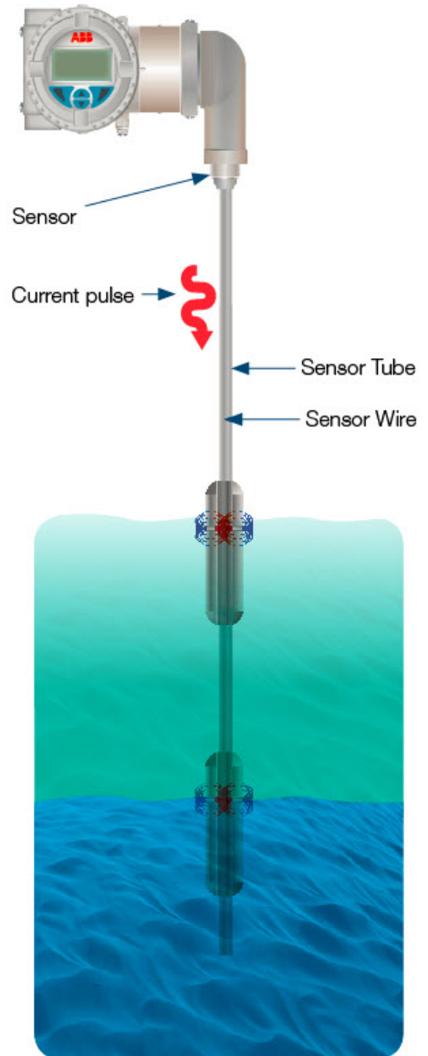
Figure 7: Magnetostrictive level transmitters use the speed of a torsional wave in a wire to produce a level measurement
